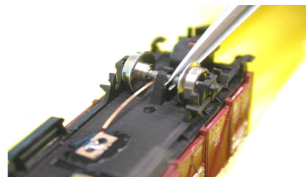
figure 5: The axle has been pushed underneath the clamp holding it in its place.
